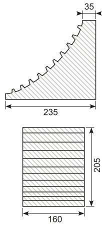
Stopklods Stop block
